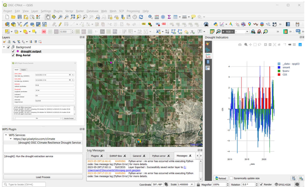
Figure 87 – View of WPS Client plugin and extracted CDI and plotted within QGIS.
