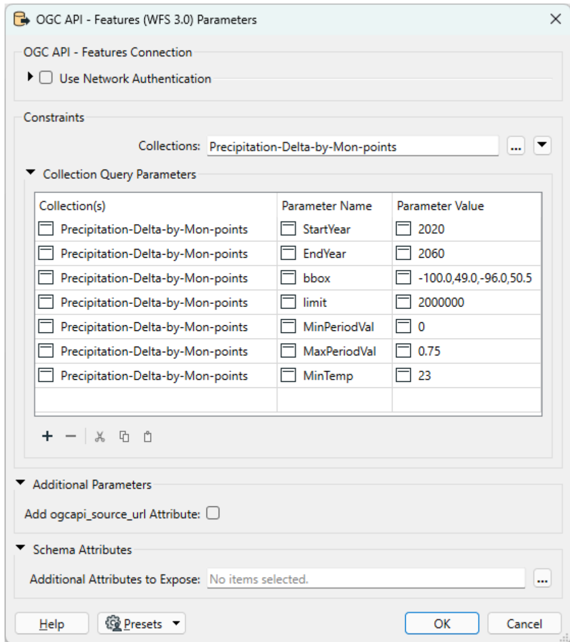
Figure 102 – OGC Features Query Parameters for mean temperature > 23C and precipitation change > 25% dryer
