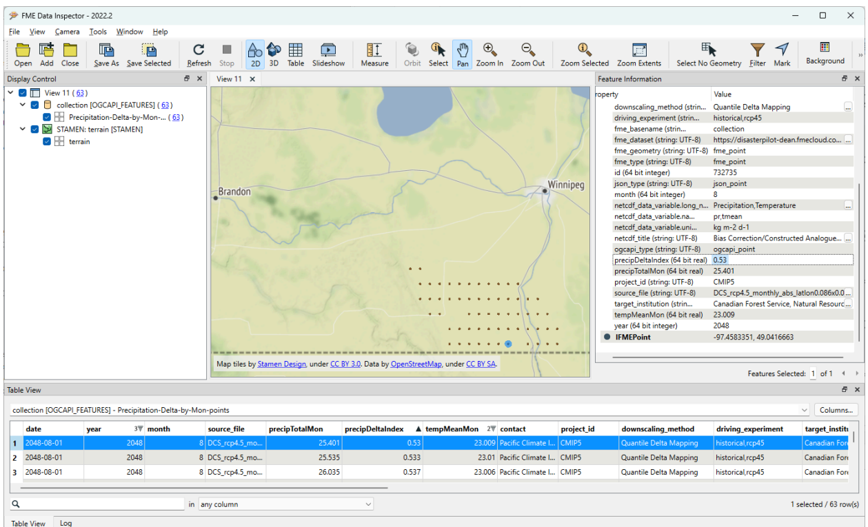
Figure 83 – FME OGC API Feature Service response as displayed in Data Inspector. Results show the response to the query below highlighting an area south of Winnipeg near the US border from August 2048 and 2058. This answers the question, “Where and when can we expect to see a drop in precipitation of more than 25% and mean monthly temperatures > 23C for the current climate scenario?”
