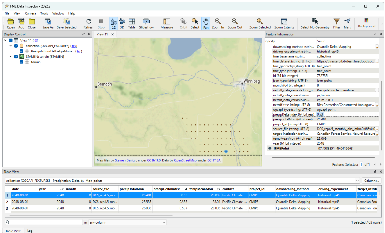
Figure 103 – OGC API Features Response to above query: 63 temporal points with associated temperature and precipitation values, as shown in FME Data Inspector client.
