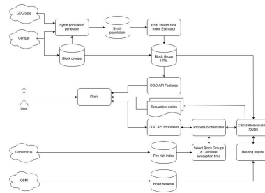
Figure 5 – D109 Technical implementation schema
