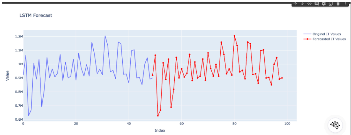
Figure 111 – Time Series Forecast.
