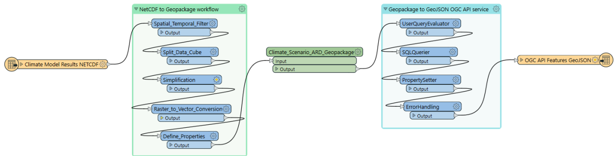
Figure 79 – High-level component FME workflow from climate data cube NetCDF to spatial database geopackage to OGC API Feature service GeoJSON.
