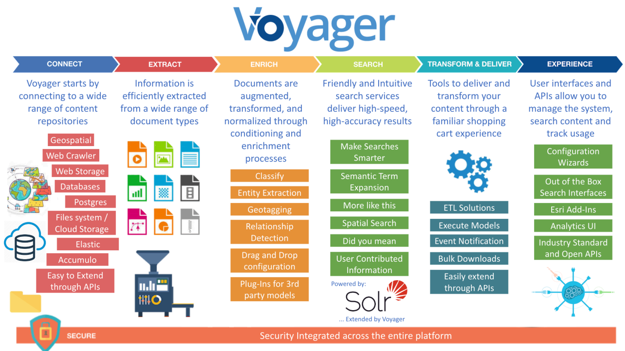
Figure 62 – Voyager Search Development and Usage Workflow.
