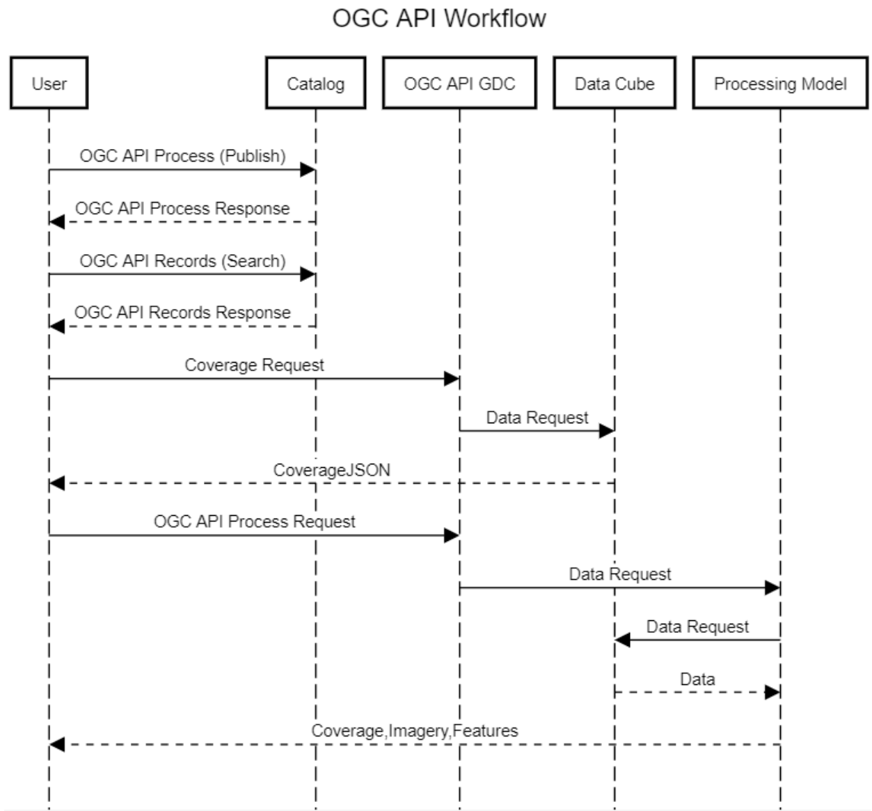
Figure 10 – Compusult OGC API Workflow
