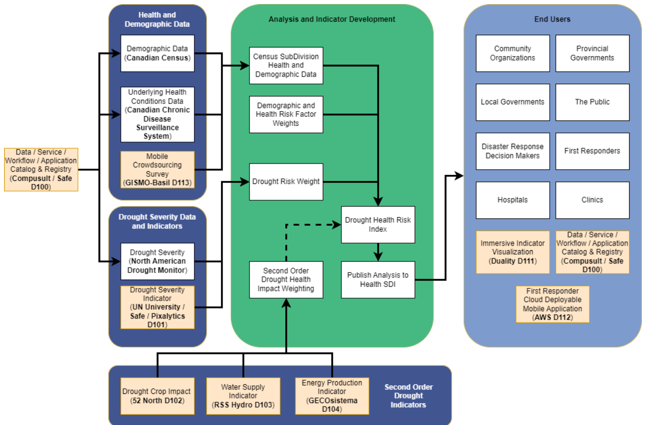
Figure 69 – Drought Health Risk Index Workflow
