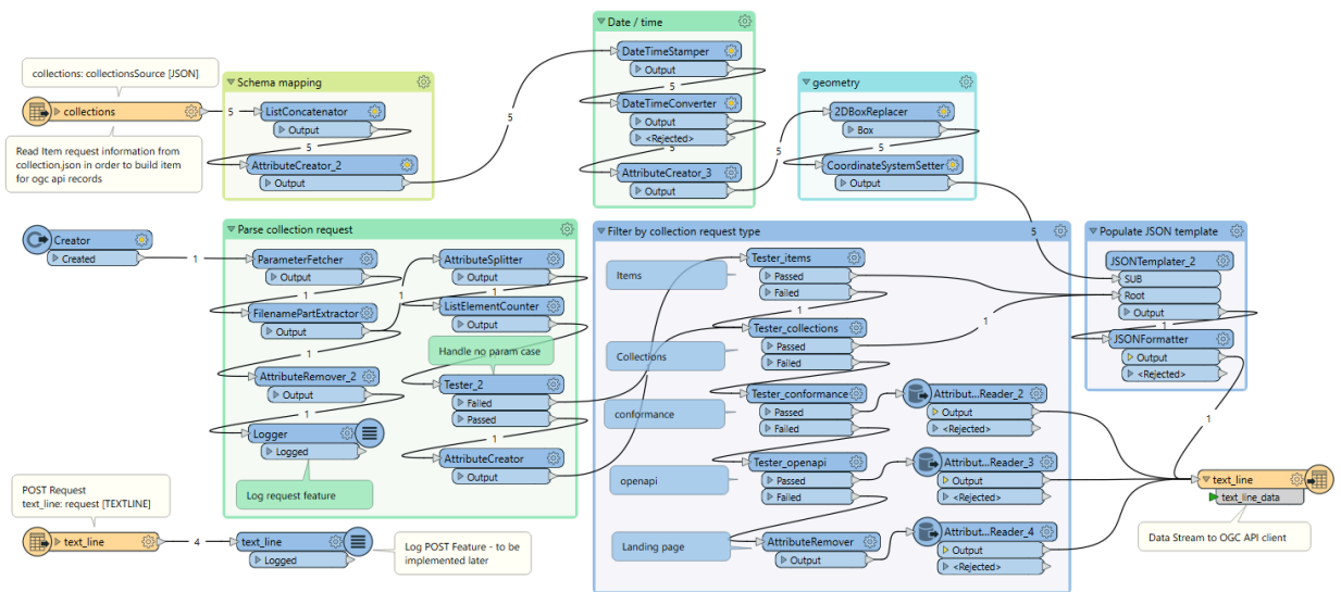
Figure 109 – OGC API Records service: message handling FME workflow
