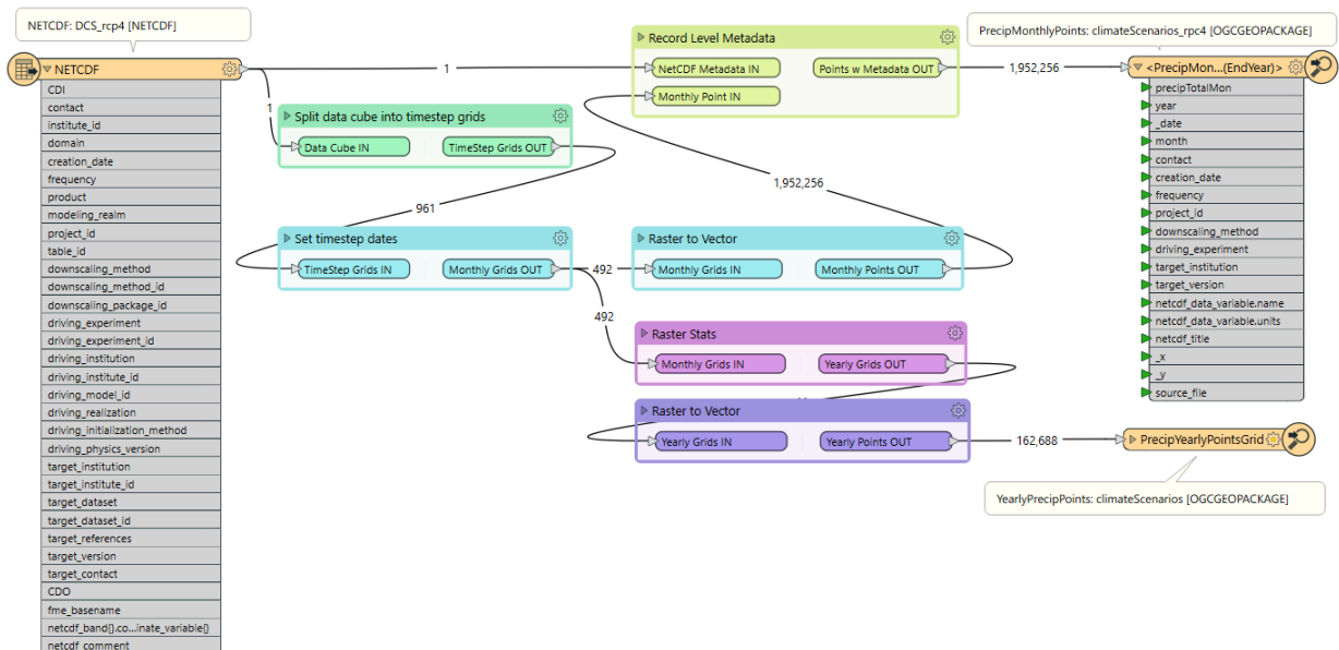
Figure 99 – Climate service data FME transformation workflow from NetCDF data cube to Geopackage relational database.
