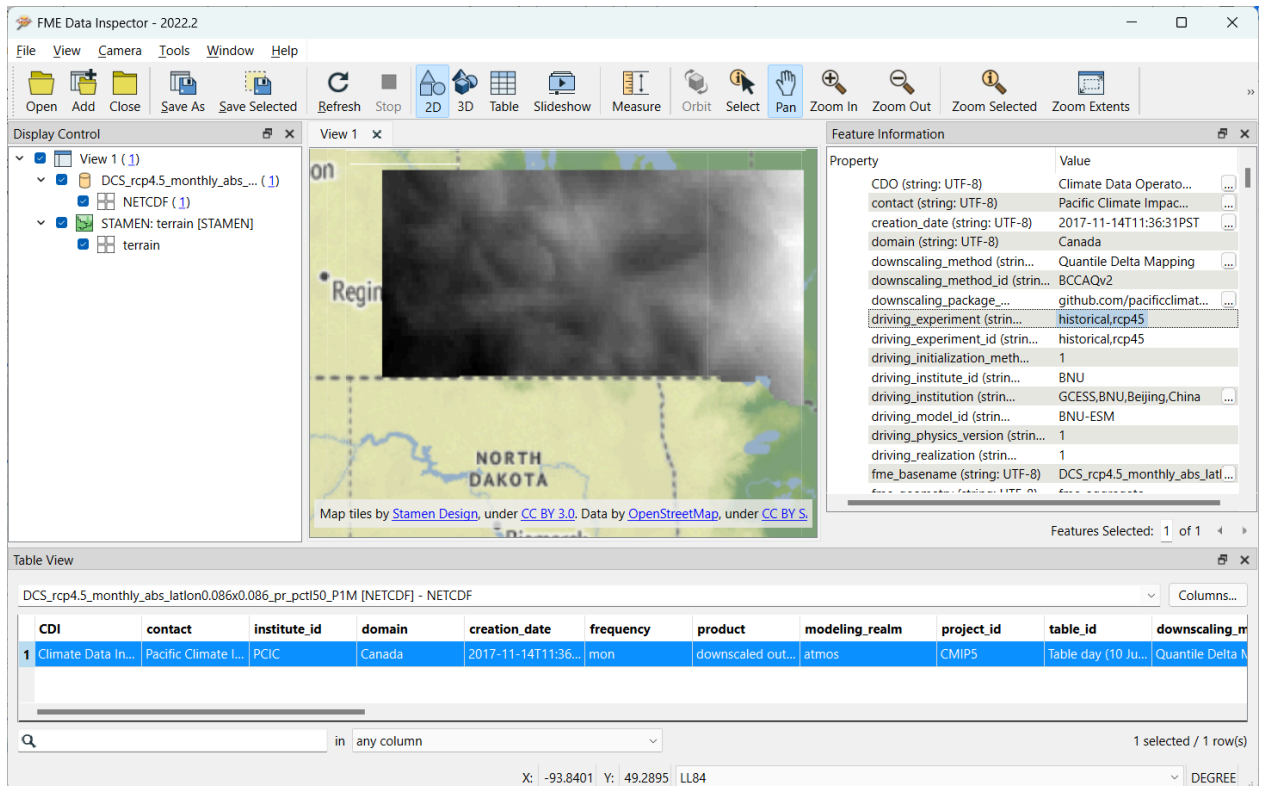
Figure 78 — Source NetCDF data cube from Environment Canada's climate data extraction tool shown in FME Data Inspector.
