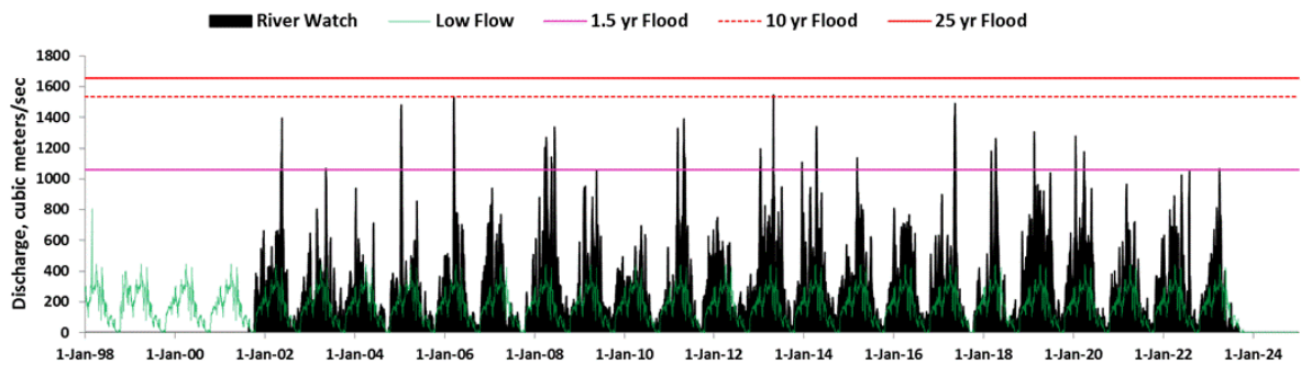
Figure 73 – Similar to Figure 72, but now showing the entire time series of water discharge using satellite data (2002 → now).
