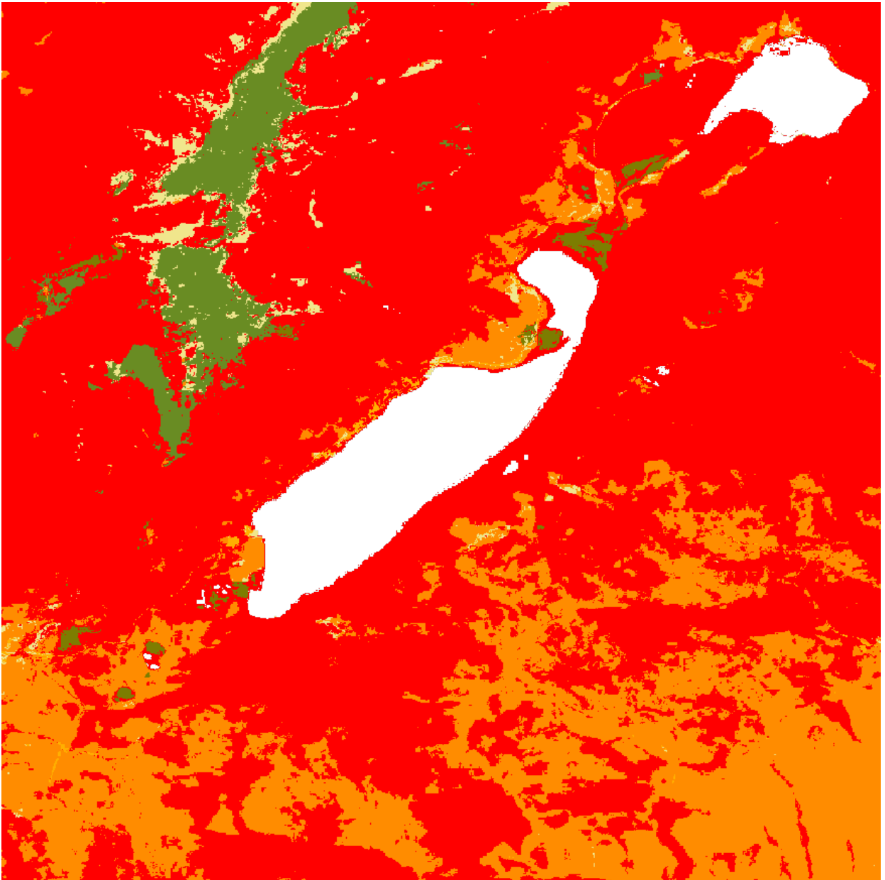
Figure 43 – Wildland Fire Fuel Indicator Workflow - Mapping predicted vegetation types to fuel density
