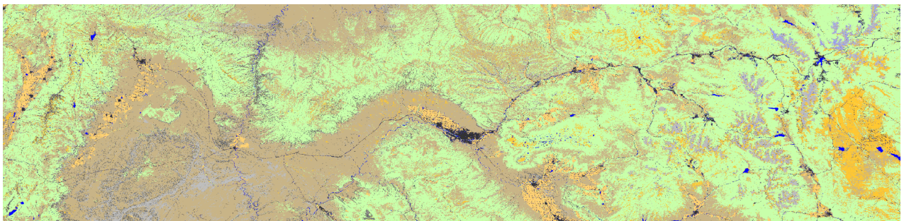
Figure 29 – Remapped High Level Fuel Vegetation Types of full training area for Fish Lake (2022)
