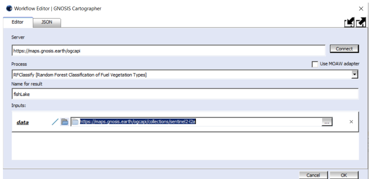
Figure 36 – Workflow Editor tool from GNOSIS Cartographer client
