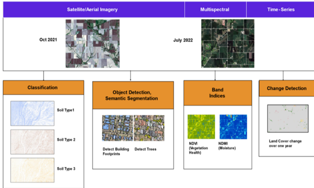
Figure 15 – Workflow with example imagery and analyses through Falcon’s GIS and AI-powered pipeline to create Digital Site Twins of the existing real locations for immersive visualization and simulation.
