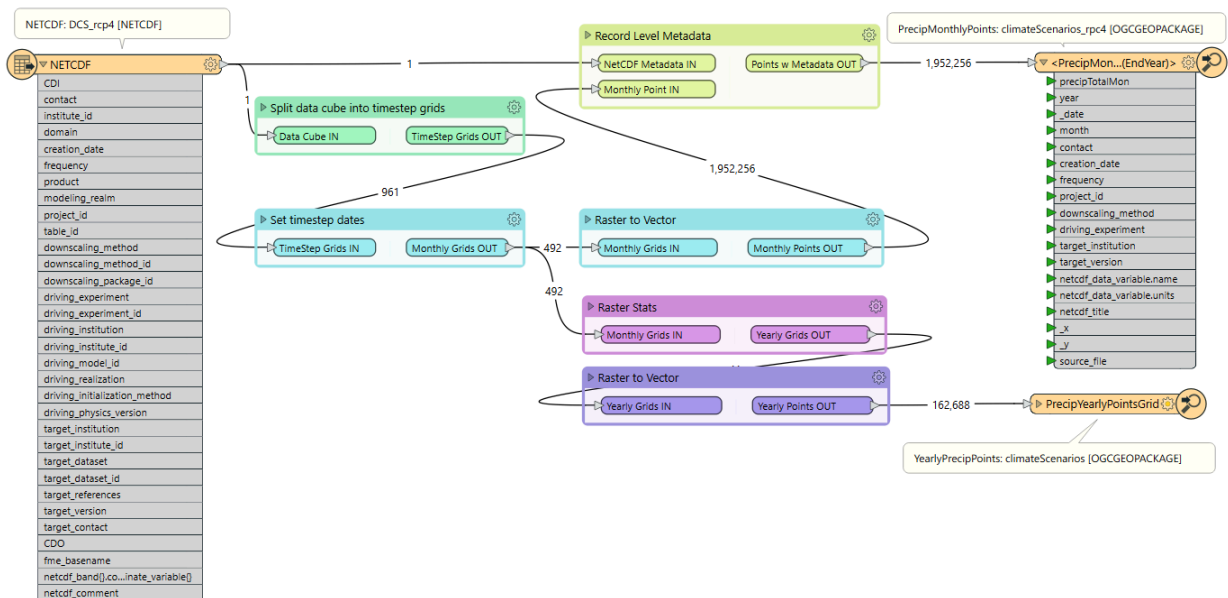
Figure 80 – Climate service data FME transformation workflow from NetCDF data cube to Geopackage relational database.
