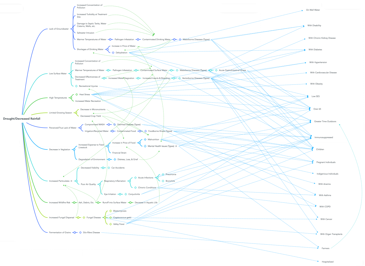
Figure 68 – Drought Health Impact Map
