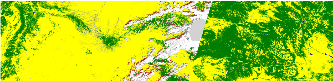
Figure 33 – Sentinel-2 SCL of training area for Fish Lake (September 15-25, 2022)
