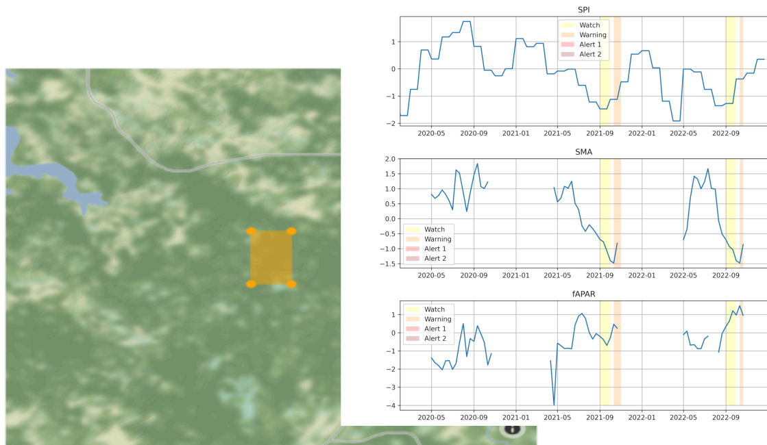
Figure 85 – Example of the Combined Drought Indicator being run for a location within Canada.
