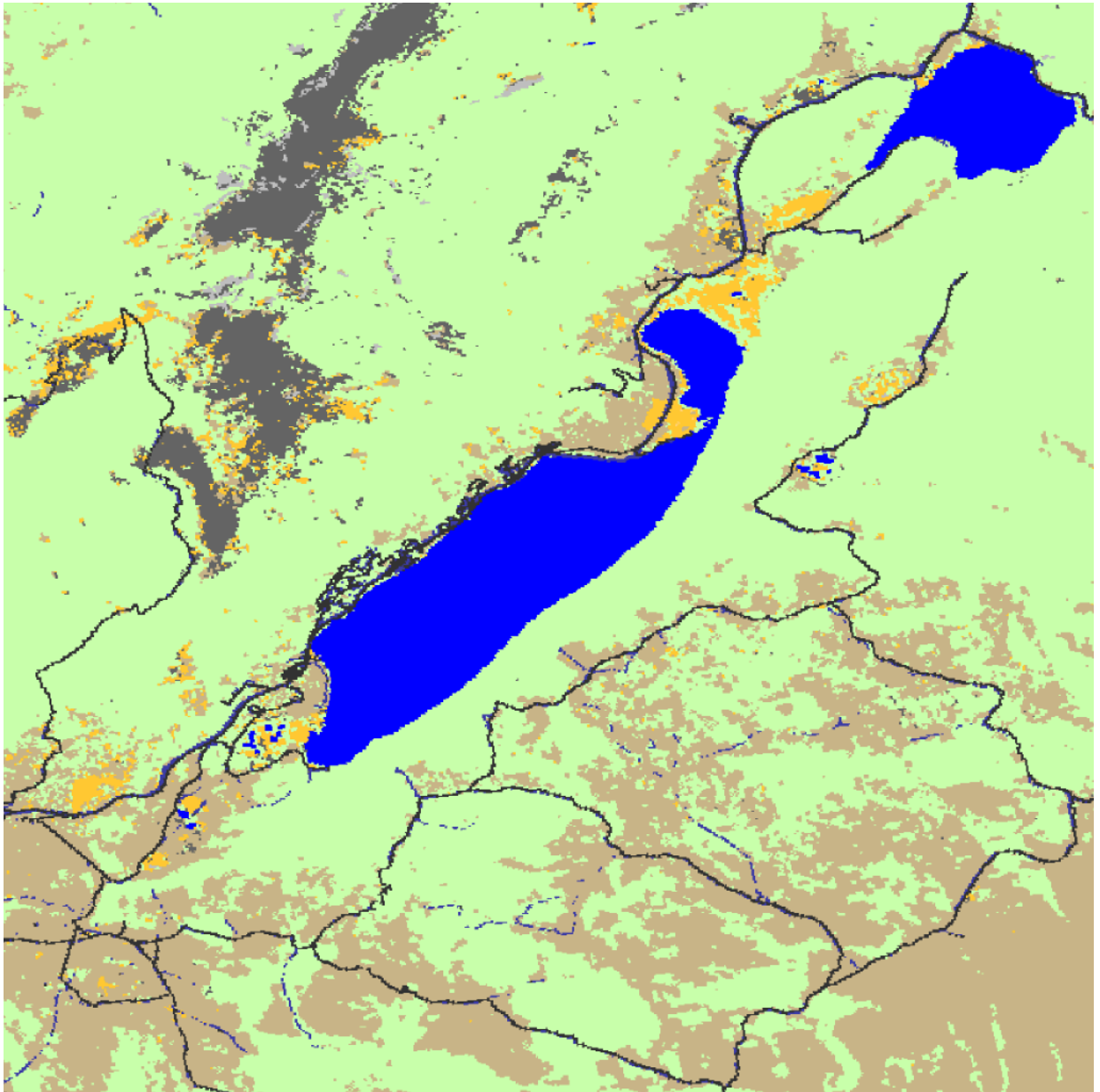
Figure 28 – Remapped High Level Fuel Vegetation Types for Fish Lake area (2022)
