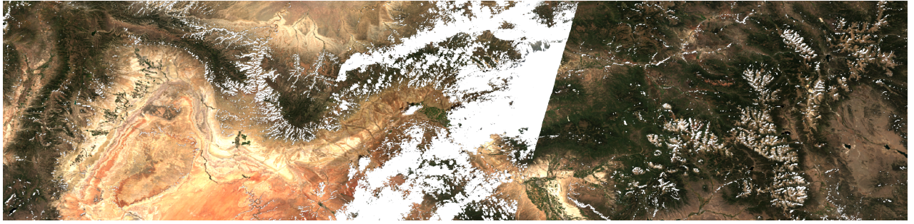
Figure 31 — Sentinel-2 Imagery of training area for Fish Lake (September 15-25, 2022)
