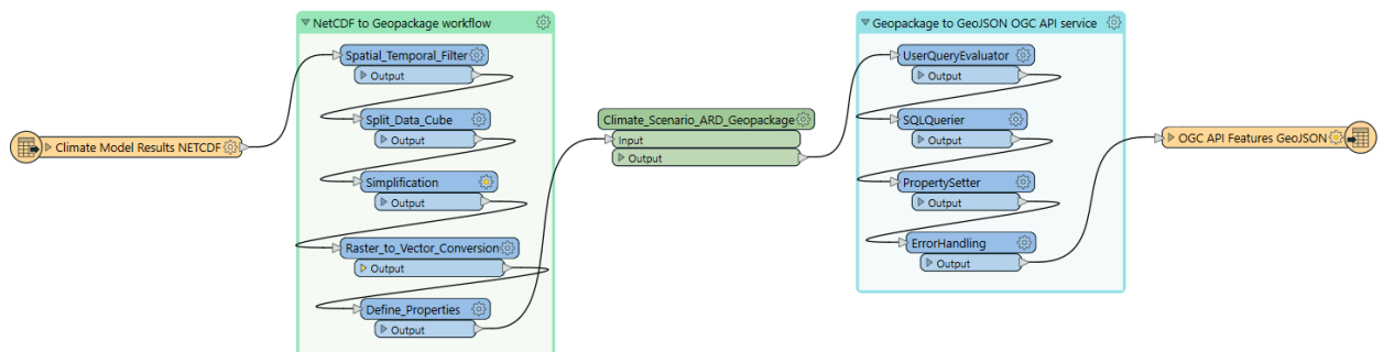
Figure 96 – High-level component FME workflow from climate data cube NetCDF to spatial database geopackage to OGC API Feature service GeoJSON.
