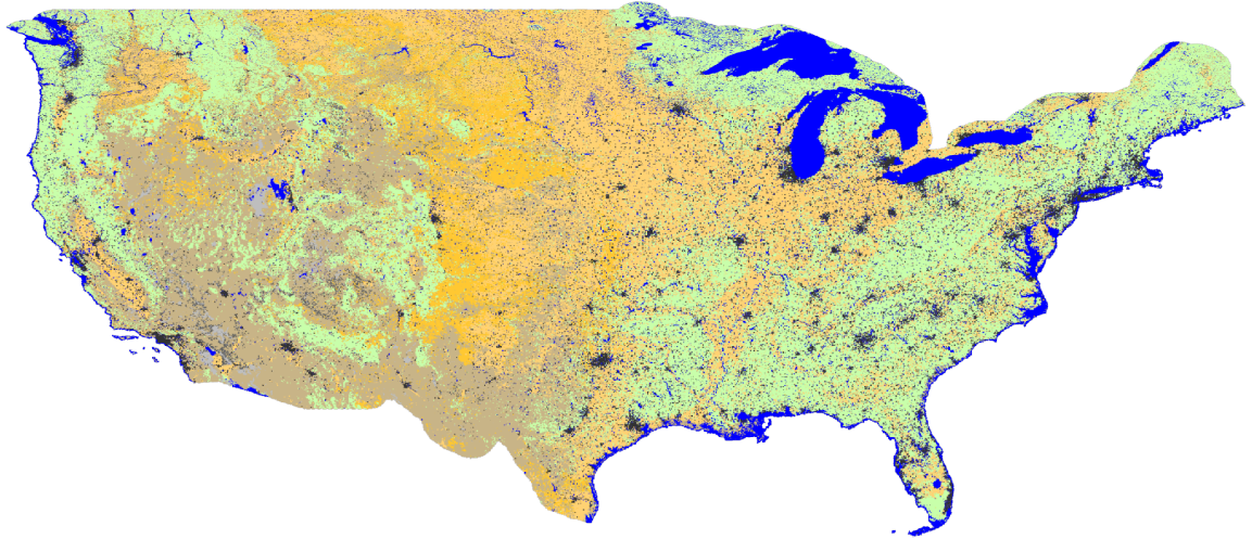
Figure 27 – Remapped High Level Fuel Vegetation Types for continental United States
