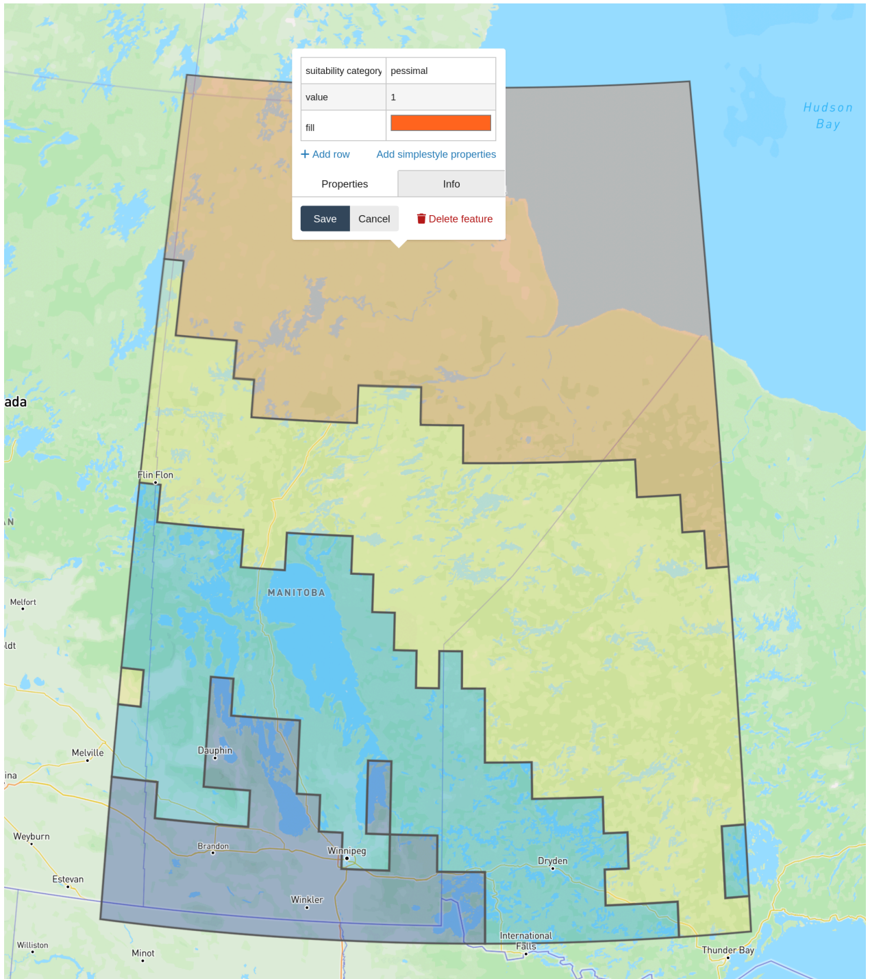
Figure 89 — Exemplary crop suitability map which is returned if calculations for a certain bounding box are requested, here for the test region in Manitoba. The suitability of the environmental conditions is decreasing from suitable (blue) to pessimal (red). This figure has been generated with the help of geojson.io .
