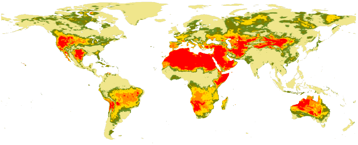
Figure 37 – CMIP5 Precipitations (from Copernicus Climate Data Store) hosted on GNOSIS Map Server
