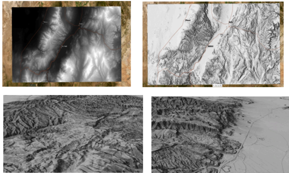
Figure 16 – Fish Lake, Utah’s Digital Elevation Model (DEM). This DEM was created by merging and resampling around 200 DEMs from USGS mapping surveys carried out in 2016, 2018, and 2020. The top left image is that of the DEM. The rest of the photos showcase DEM’s 3D Hillshade views covering various parts of the terrain.
