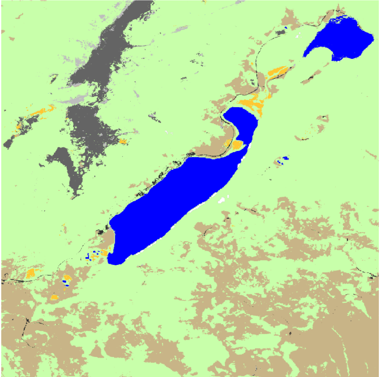
Figure 40 – Wildland Fire Fuel Indicator Workflow - Predicted high level fuel vegetation types (Fish Lake, 2022)
