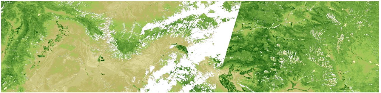
Figure 35 – Sentinel-2 EVI of training area for Fish Lake (September 15-25, 2022)
