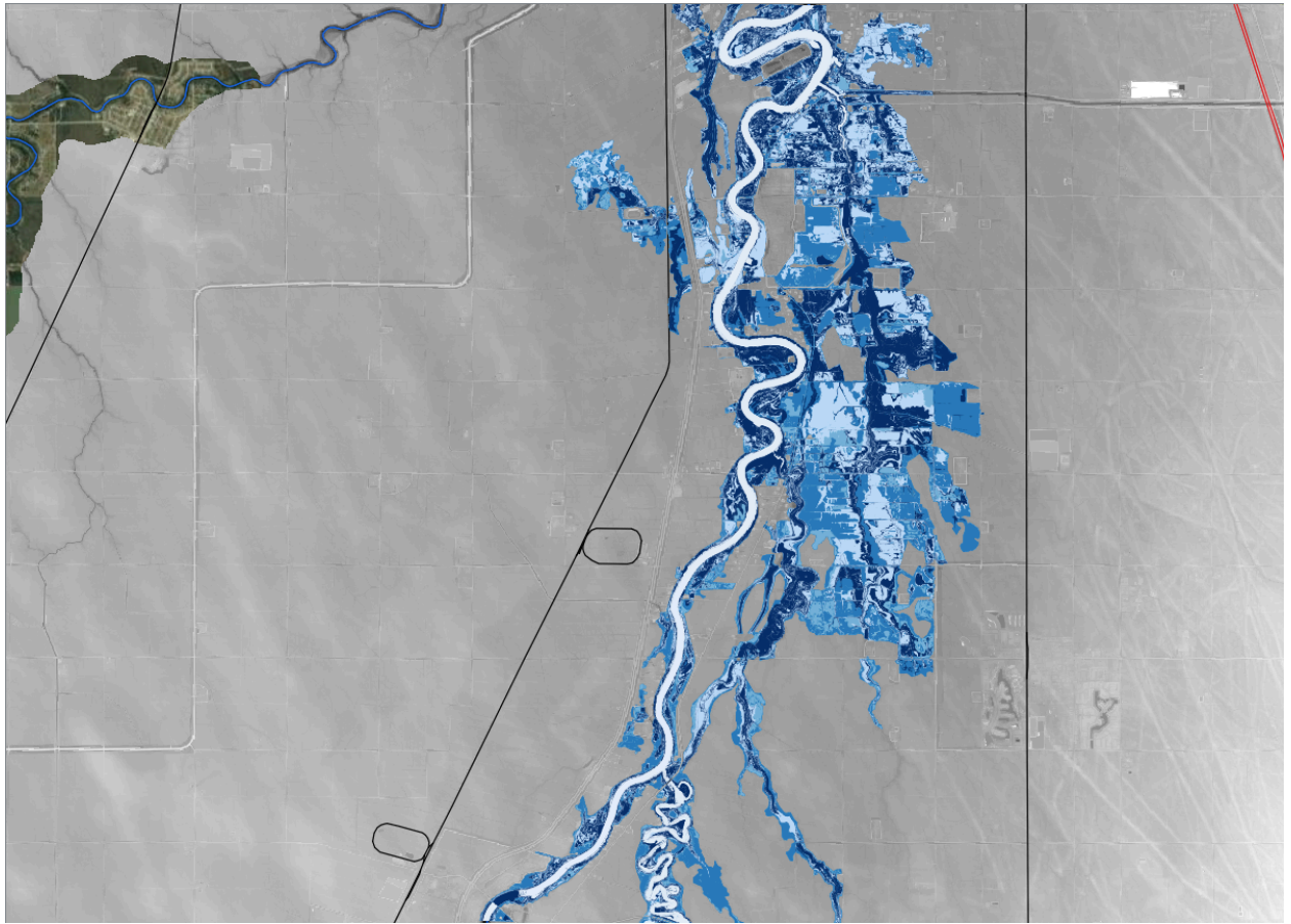
Figure 18 – Area of 2011 flooding, colored light to dark blue according to flood day (start to end) overlaid on DEM (shades of gray), with railway line as black lines, and motorway as a red line; flooding area from RSS Hydro.
