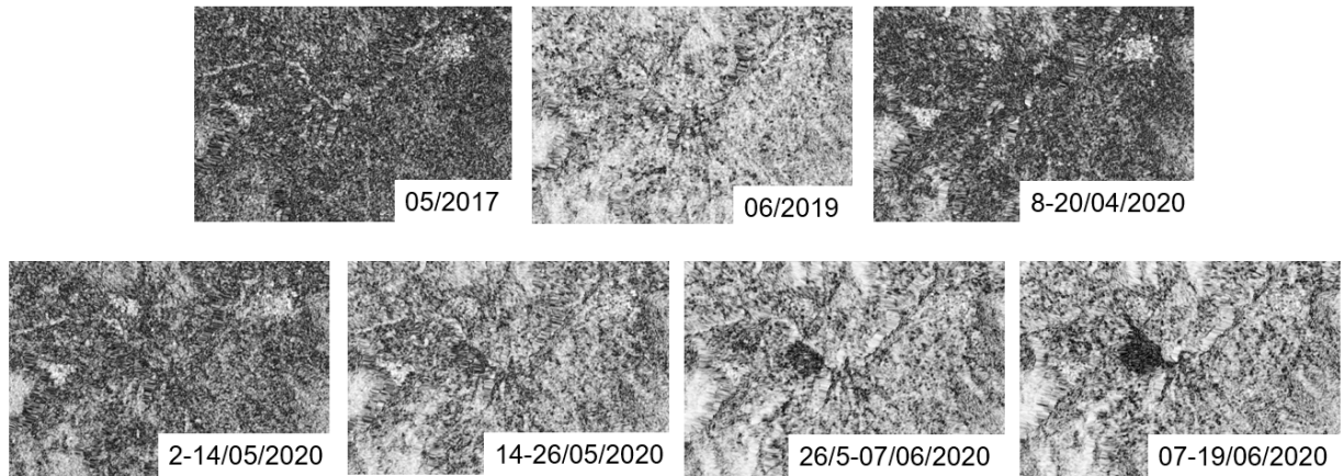
Figure 16 – Time series of coherences generated with Sentinel-1 data over Achoma.
