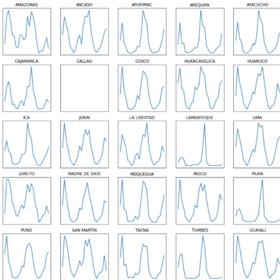
Figure 7 – Precipitation in different Peruvian regions 2016-2018; generated by SatCen.
