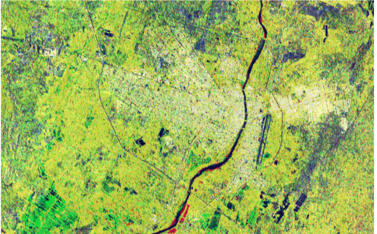
Figure 11 – Example of MTC product generated with Sentinel-1 over Piura. Red areas close to the rivers highlight the flooded area during the period; generated by SatCen.
