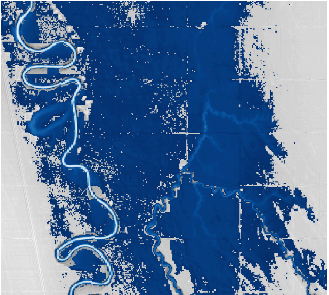
Figure 19 – Section of the April 2020 flooding, colored dark to light blue according to occurrence, developed by Wuhan University, overlaid on the DEM.
