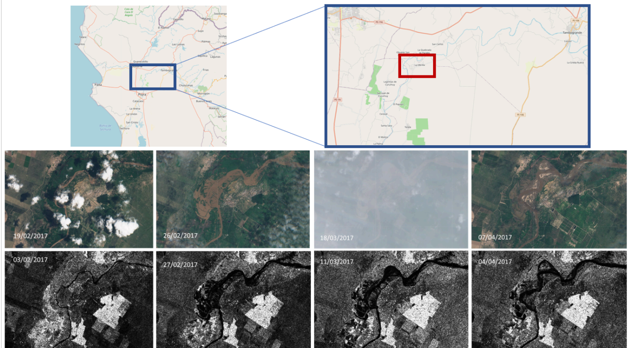
Figure 9 – Sentinel-1 (SAR) and Sentinel-2 (optical) during the flood event 2017; generated by SatCen.
