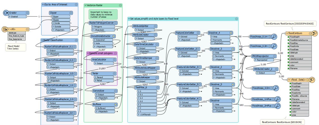
Figure 20 – ETL approach for converting flood area grid ARDs to flood contour IRD using FME from Safe Software
