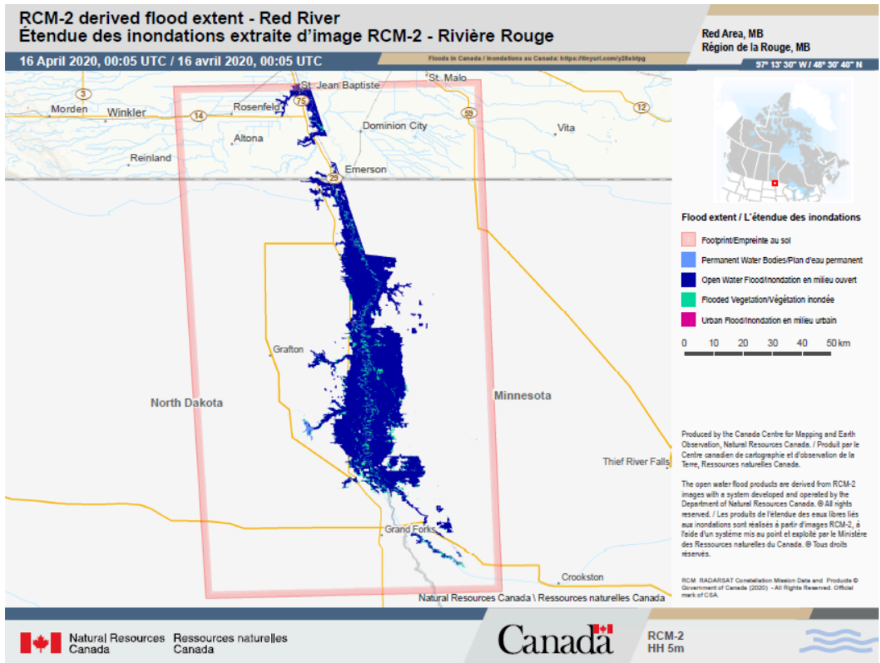
Figure 17 – RADARSAT Constellation Mission-2 derived Red River flood extent for April 2020; example courtesy of NRCan.
