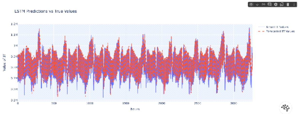
Figure B.12 – Model's actual vs predicted values
